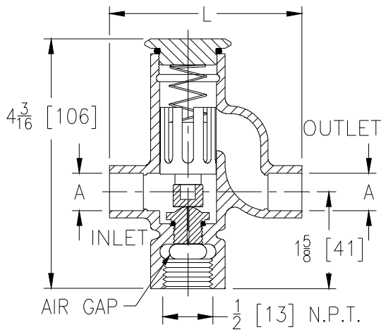
1/2 [13] PIPE SIZE
