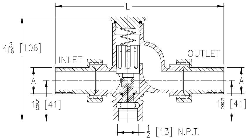
3/4 [19] PIPE SIZE
