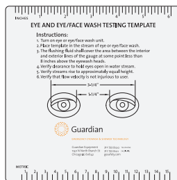
Eyewash Tester
