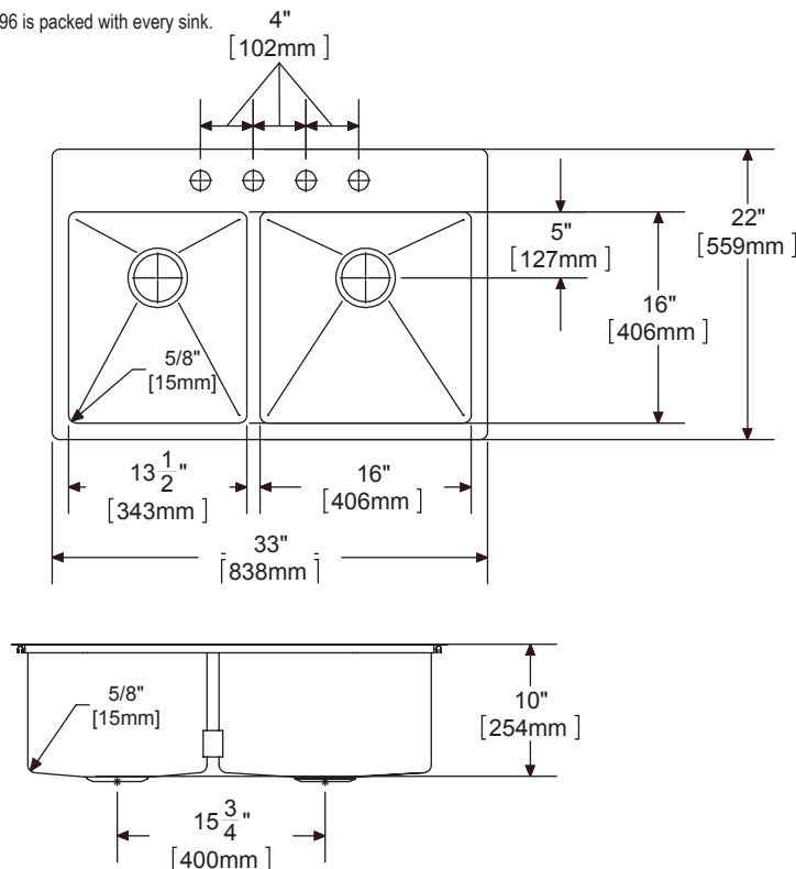
Model EFRTUO332210L4 Illustrated
