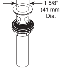
RP81628▲ Push Button Drain with overflow holes
