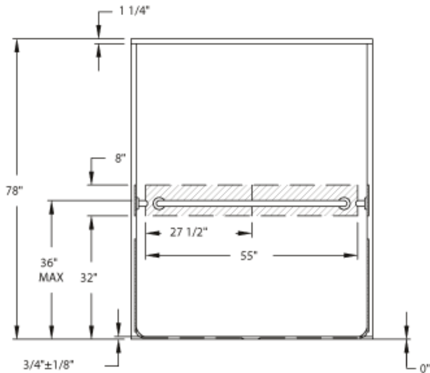
FRONT VIEW
