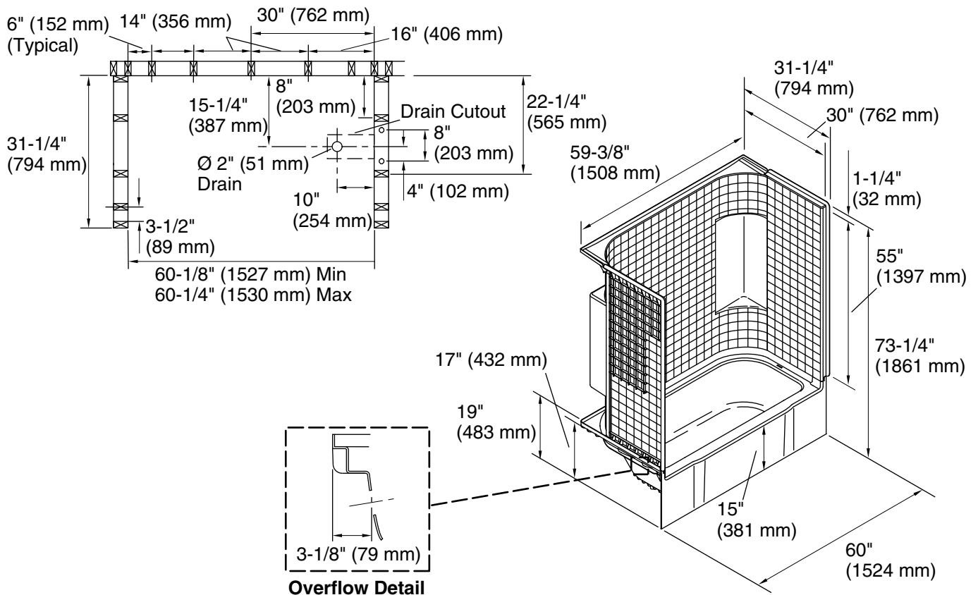
Product Diagram
