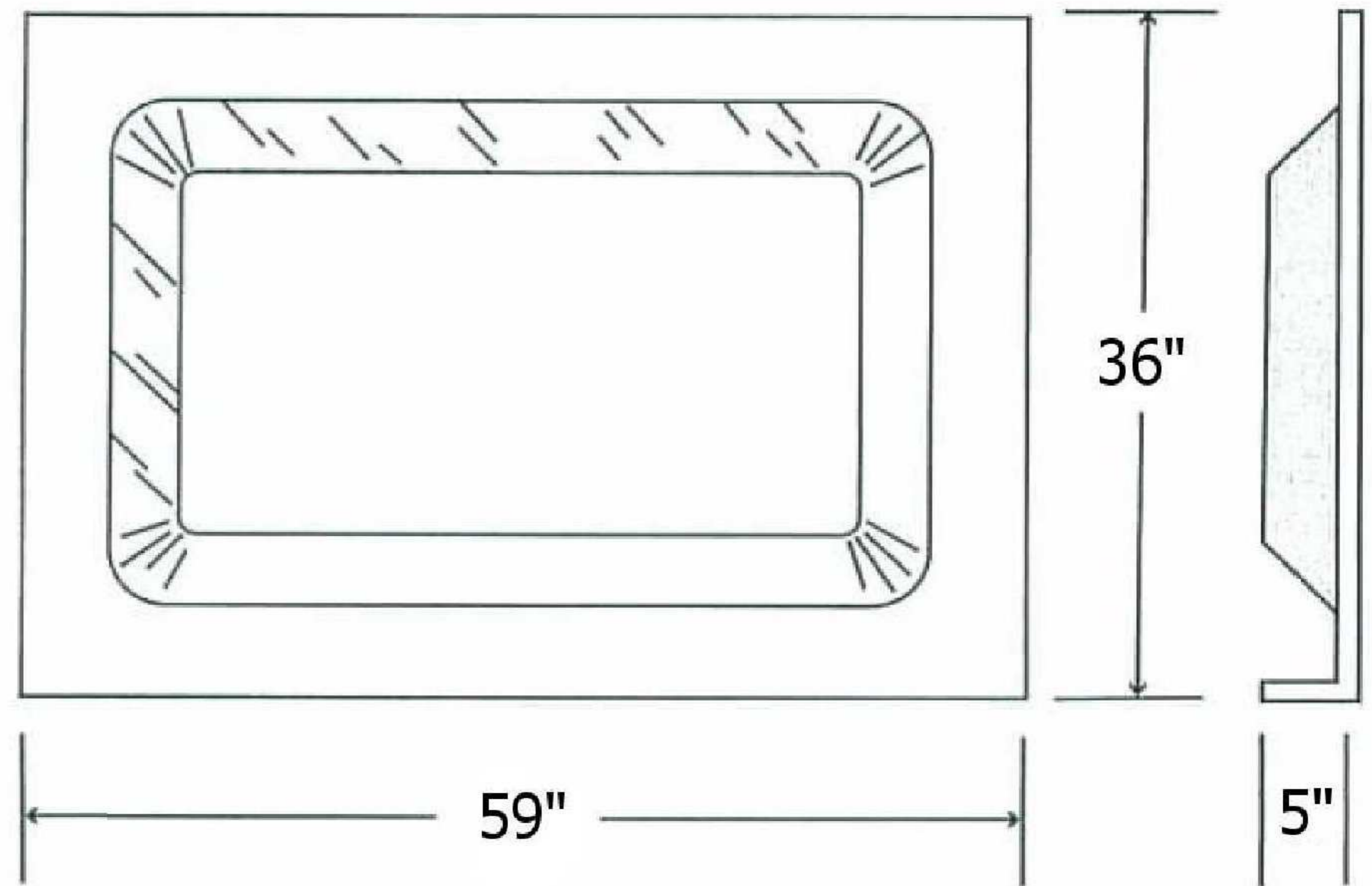
MODEL 60T DOME
