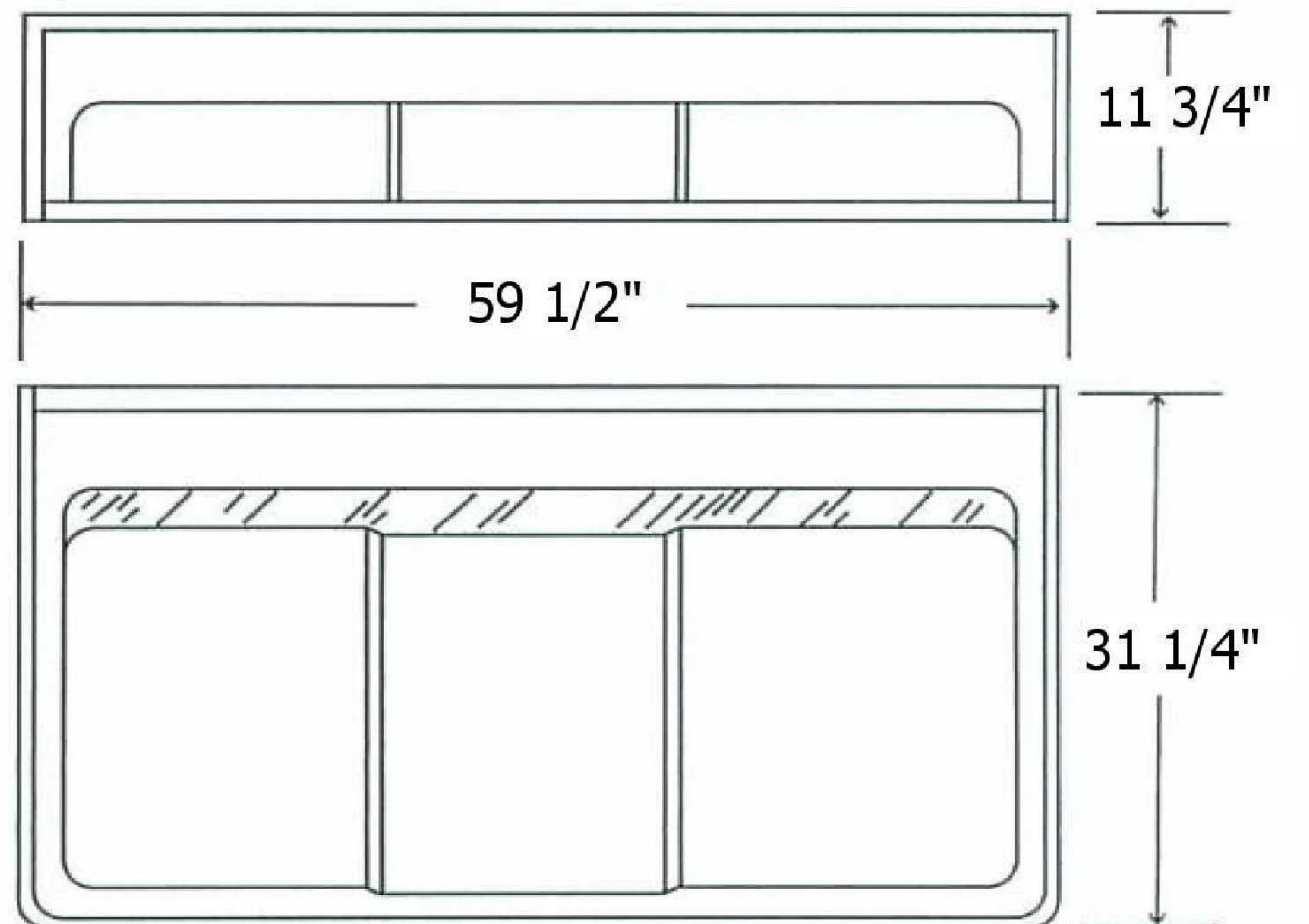
MODEL 60-30T DOME
