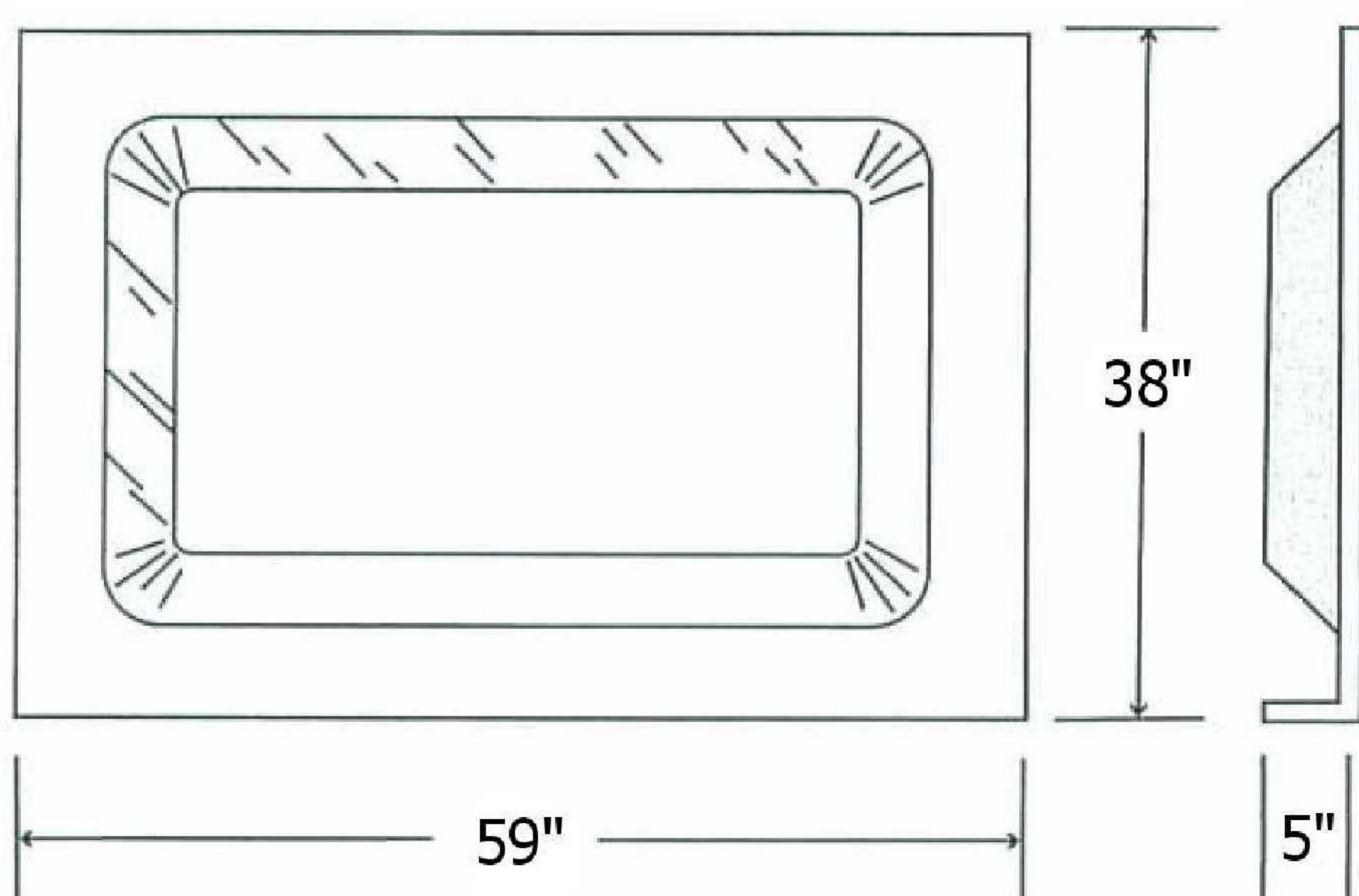
MODEL 60S DOME
