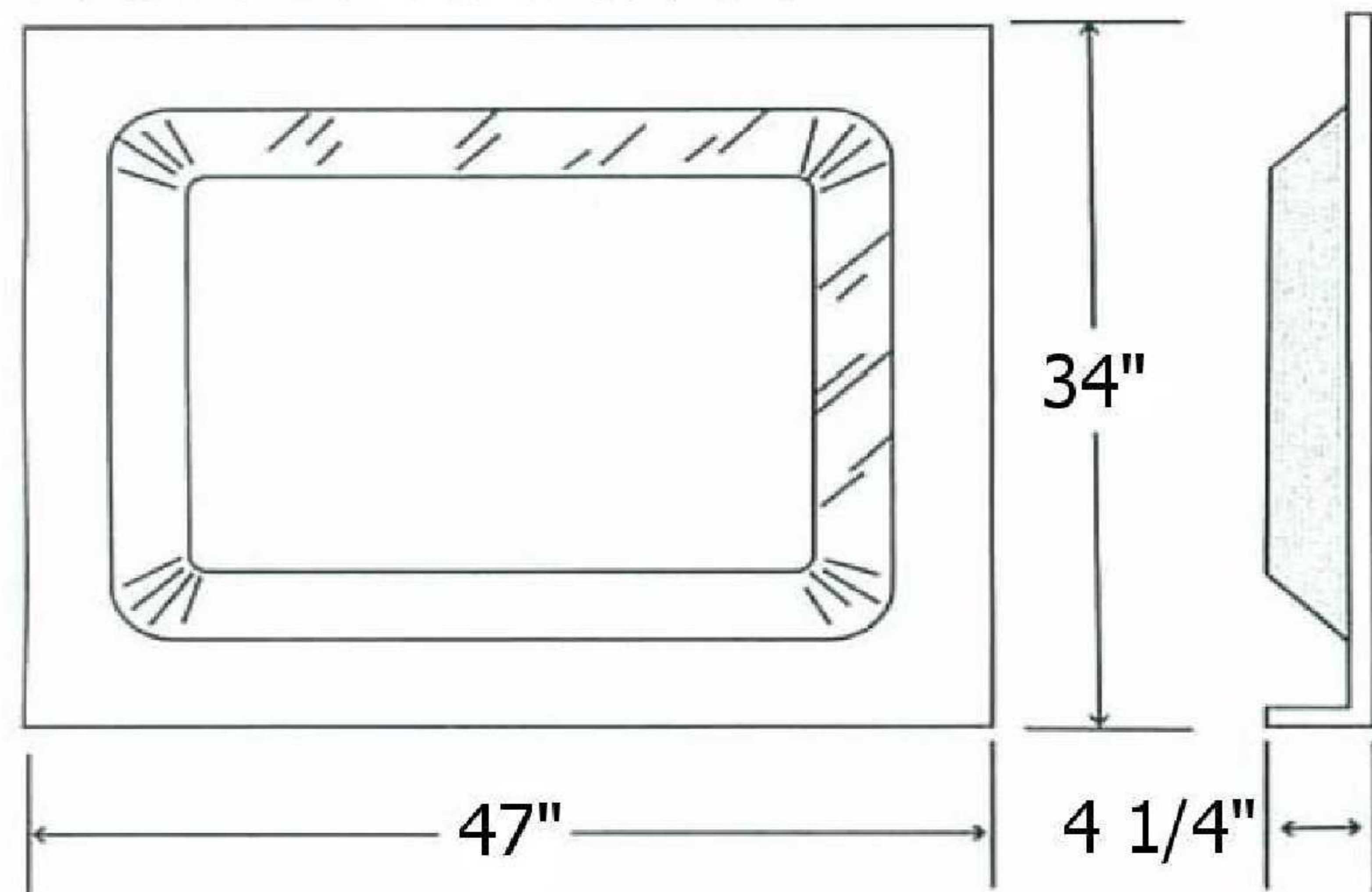
MODEL 48 DOME
