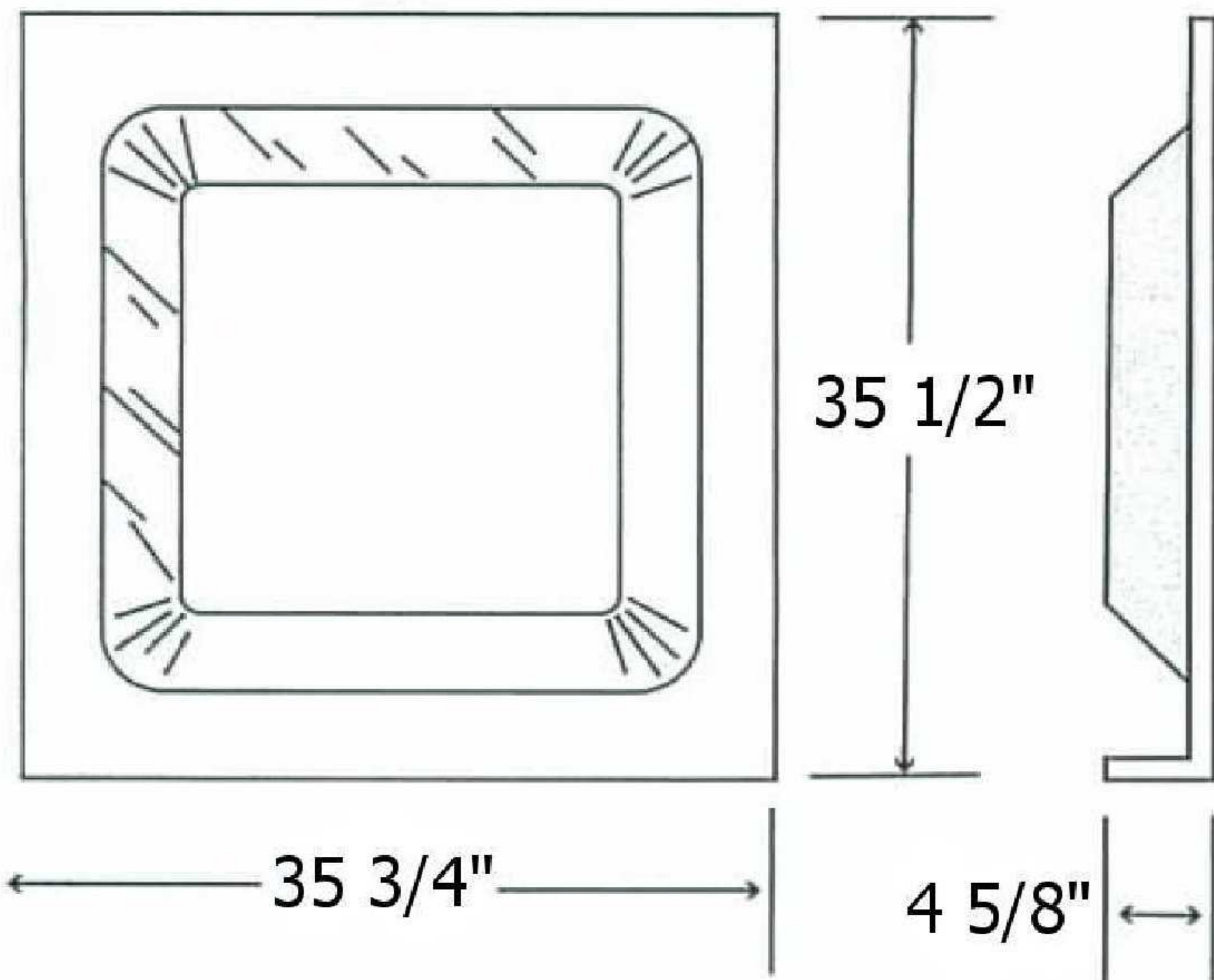
MODEL 36 DOME
