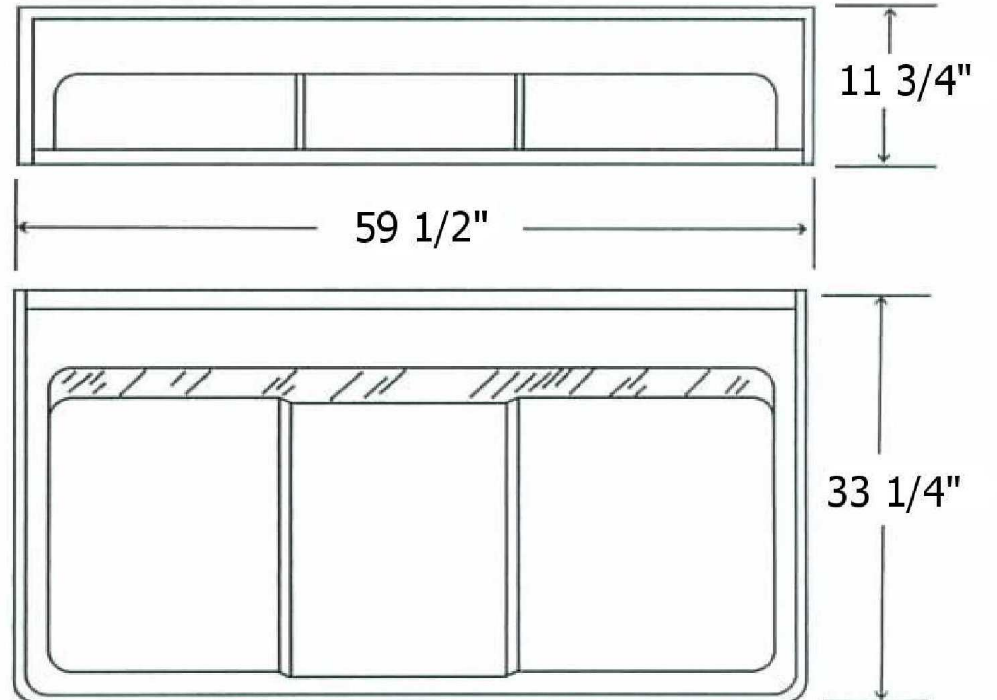
MODEL 60T DOME
