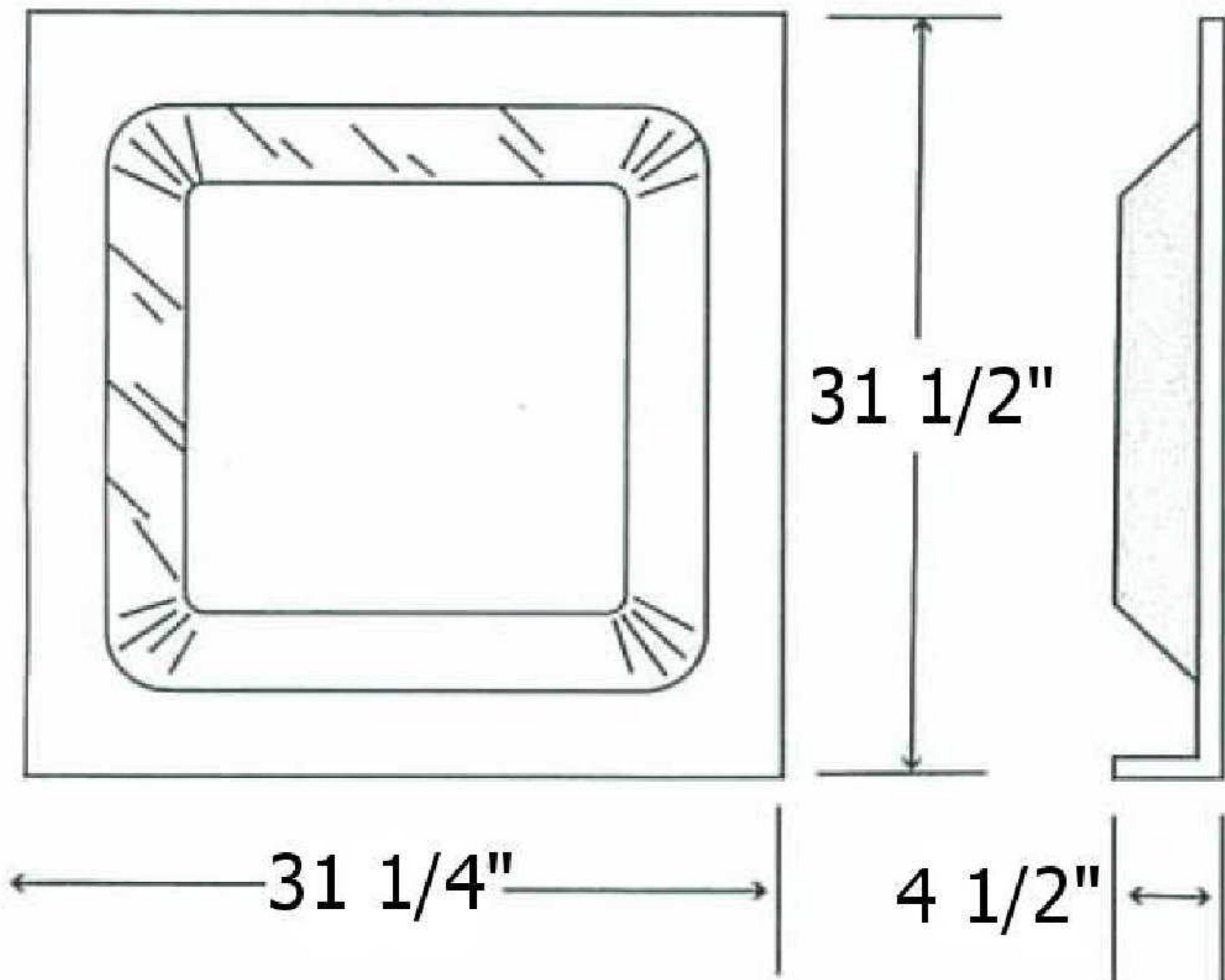
MODEL 36 DOME
