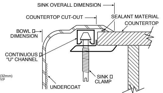
Camelot® Double Bowl Bar Sink Model: 22235 (KSR-2518-1-WF)
