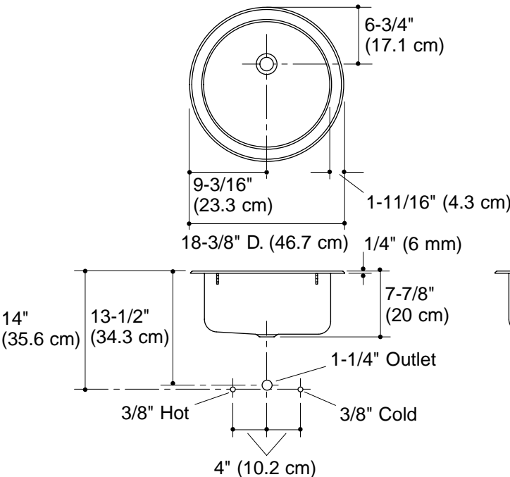
Self-Rimming Installation
