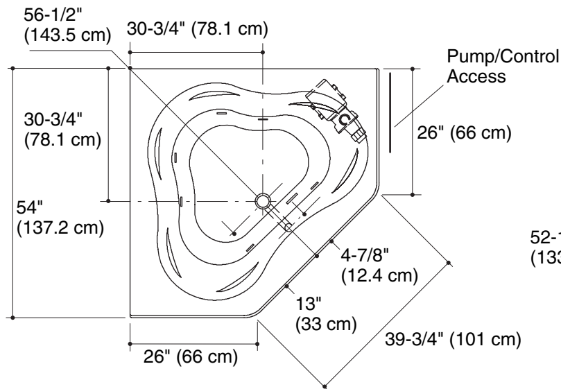
Drop-in Rim Style Cut-out Detail
