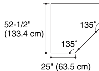
Drop-in Rim Style Cut-out Detail
