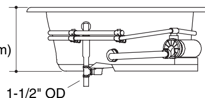
Drop-in Rim Detail
