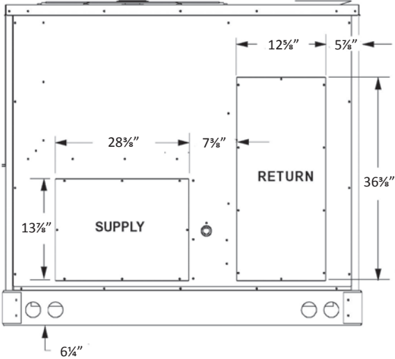
Horizontal Discharge
