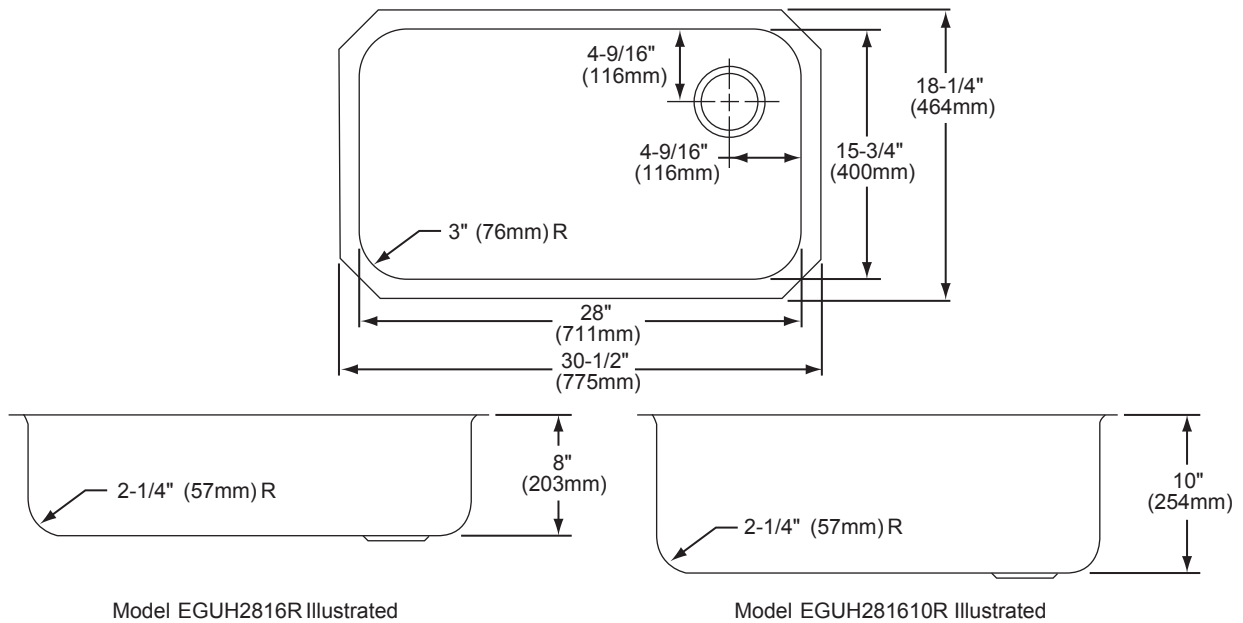
Model EGUH2816R Illustrated
