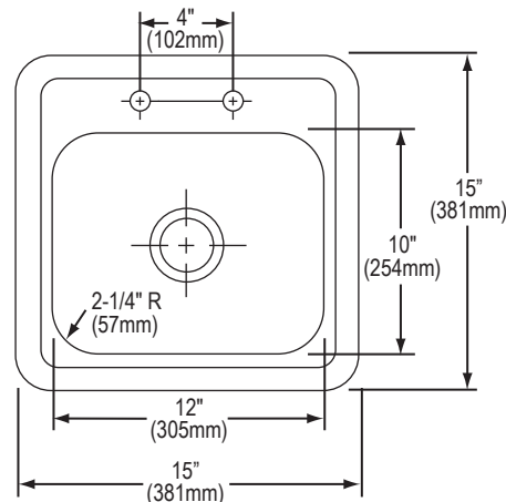
Bowl Depth is 5-1/8" Model D115152 Illustrated
