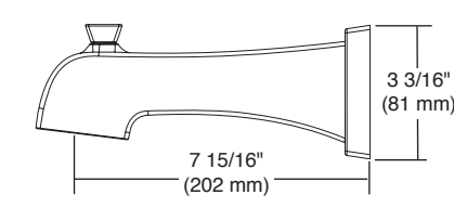
RP77092▲ (Non Diverter)
