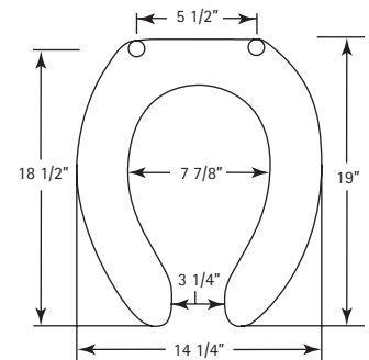
Ring thickness is 13/16" Ring thickness including the bumper is 1
