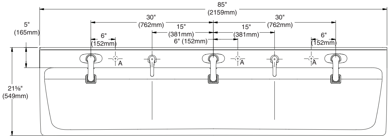
Top View (shown with shared soap option)
