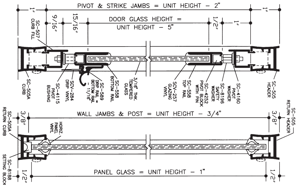
VERTICAL CROSS SECTION
