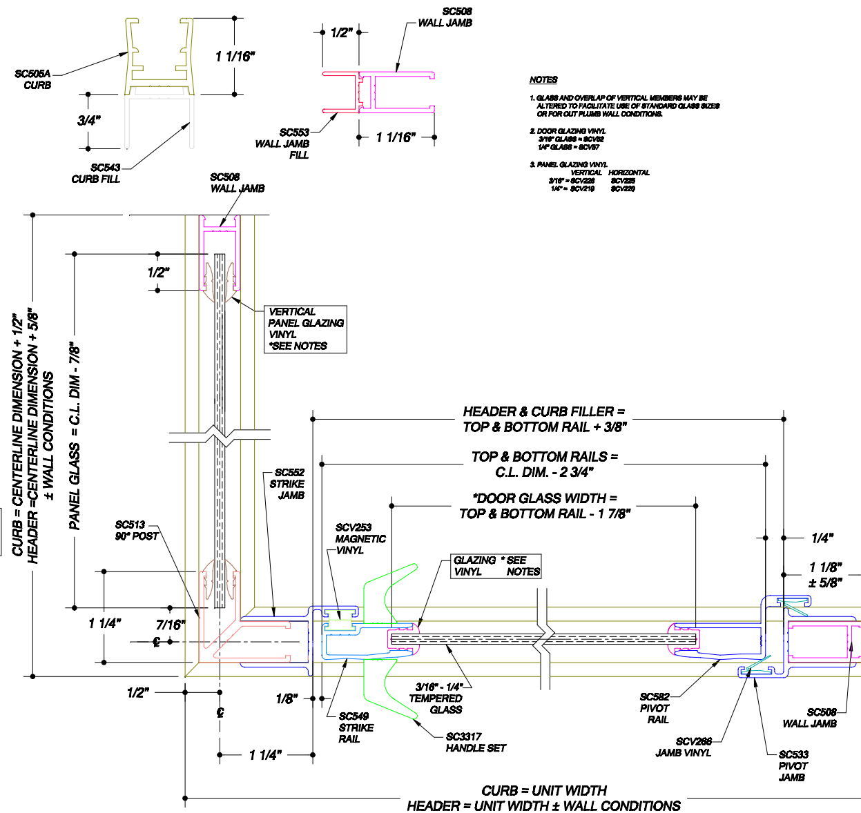
HORIZONTAL CROSS SECTION
