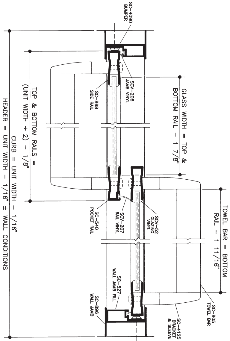
HORIZONTAL CROSS SECTION
