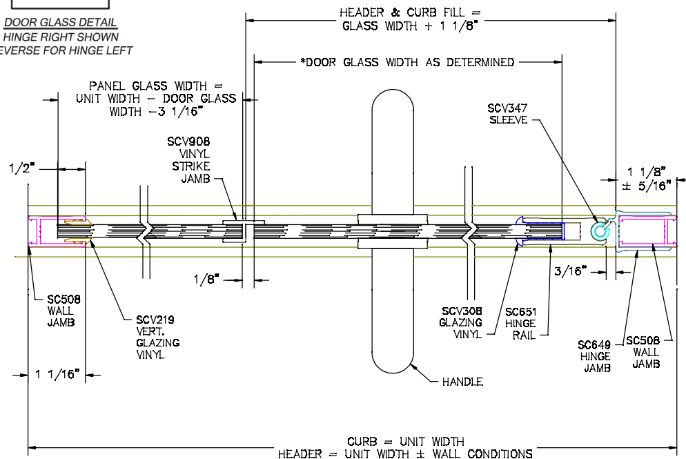
HORIZONTAL CROSS SECTION
