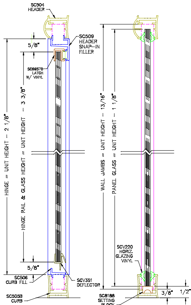
VERTICAL CROSS SECTION
