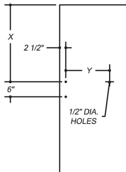
DOOR GLASS DETAIL HINGE RIGHT SHOWN REVERSE FOR HINGE LEFT
