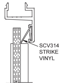
STRIKE JAMB DETAIL MAGNET WITH VINYL
