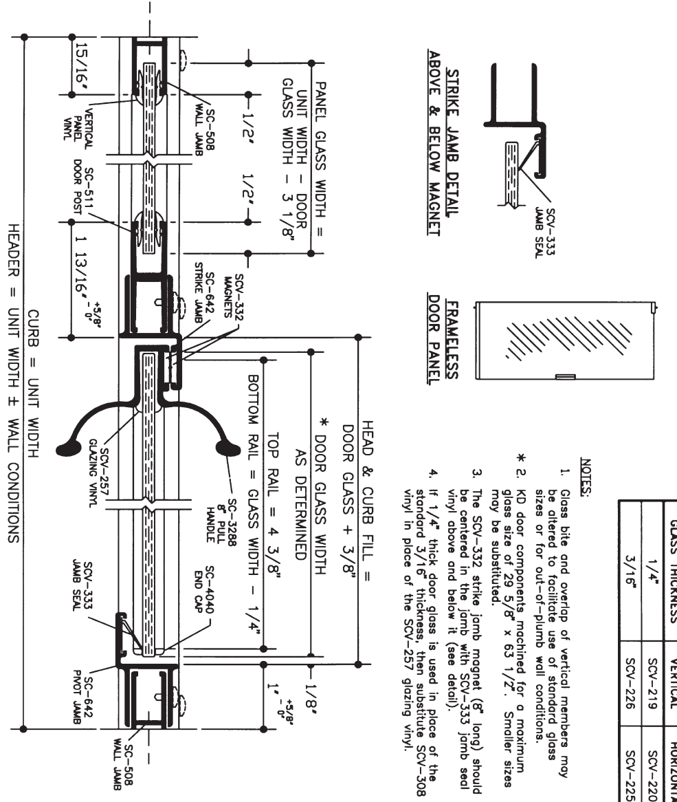
HORIZONTAL CROSS SECTION
