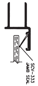
STRIKE JAMB DETAIL ABOVE & BELOW MAGNET
