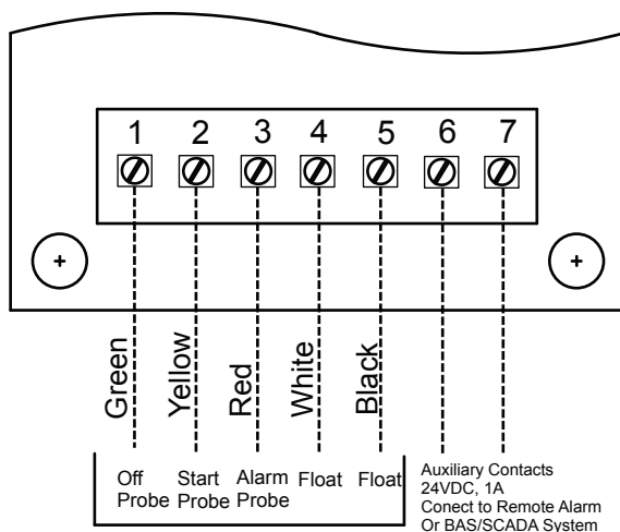
Figure 6 Circuit Board
