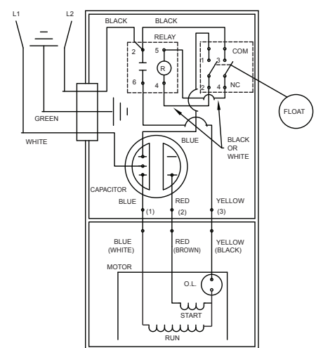
WIRING DIAGRAM FOR MODELS "M163-D" thru "M163-H" "D163-D" and "M163E" 9/86 (VS) to current
