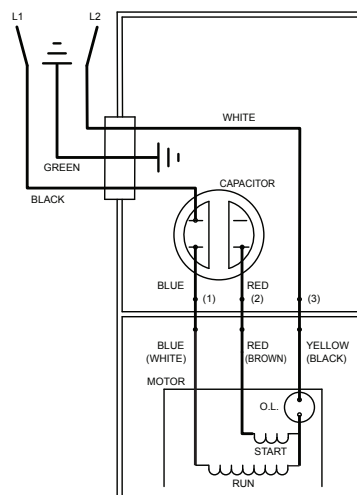
WIRING DIAGRAM FOR MODELS "N163-B" thru "N163-H" "E163-B" thru "E163-E" 1/83 (MD) to current
