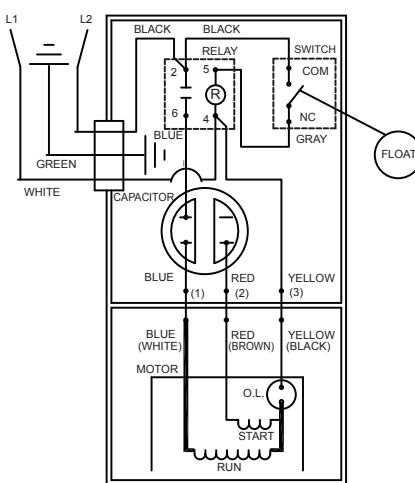
WIRING DIAGRAM FOR MODELS "M163-B" and "M163-C" "D163-A", "D163-B", "D163-C" 1/83 (MO) thru 8/86 (US)
