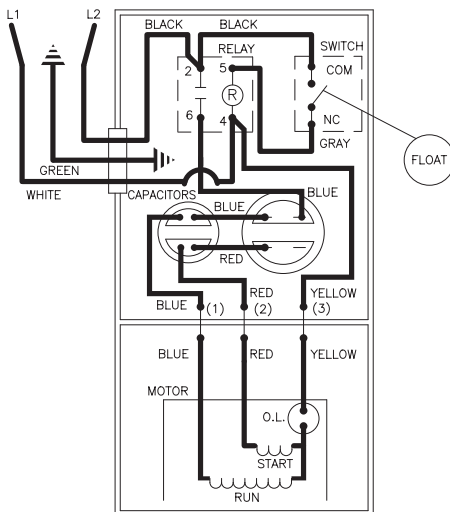
WIRING DIAGRAM FOR MODELS "M163-A" 4/81 (PM) thru 12/82 (YN)
