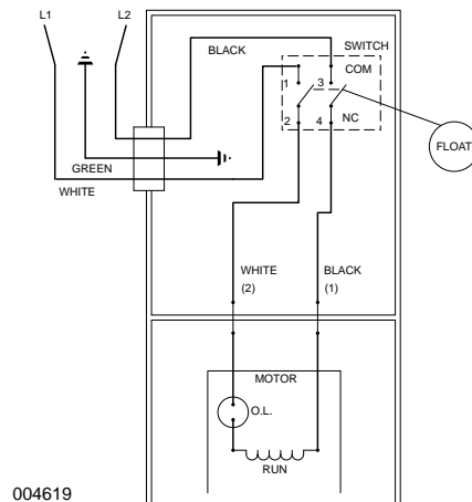
WIRING DIAGRAM FOR MODELS "M57-C", "M57-D" and "M57-E" "D57-C", "D57-D" and "D57-E" 9/86 (VS) thru Current
