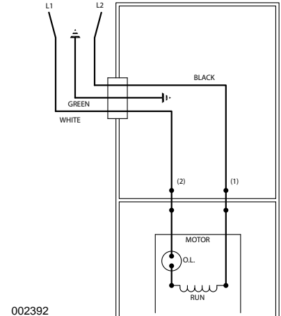
WIRING DIAGRAM FOR MODELS "N57", "N57-A", "N57-B", "N57-C", "N57-D" "E57", "E57-A", "E57-B", "E57-C", "E57-D" 8/79 (UI) thru Current
