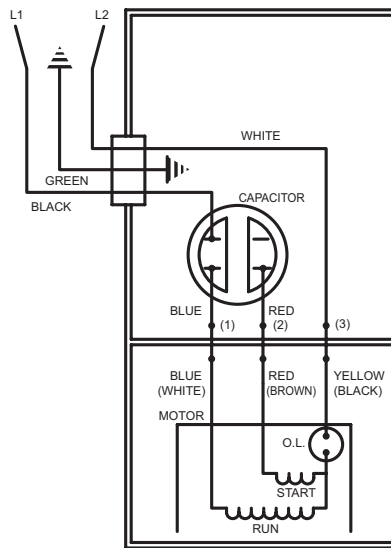
WIRING DIAGRAM FOR MODELS "I295-A", "I295-B" and "I295-C" 5/86 (RS) to Current
