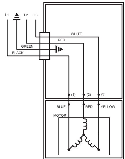
WIRING DIAGRAM FOR MODELS "J295", "F295", "G295" and "BA295" All Revisions 1/86 thru Current
