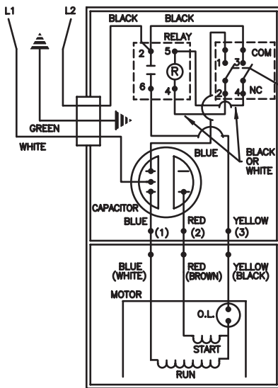
WIRING DIAGRAM FOR MODELS "H295-A", "H295-B" and "H295-C" 5/86 (RS) to Current
