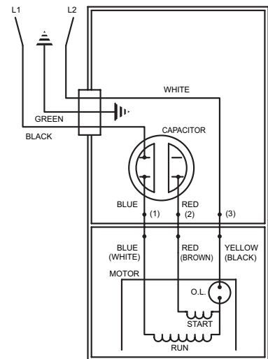
WIRING DIAGRAM FOR MODELS "E294-A", "E294-B", "E294-C", "E294-D", "E294-E" and "E294-F" 2/85 (NR) thru Current
