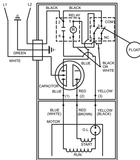
WIRING DIAGRAM FOR MODELS "D294-C", "D294-D", "D294-E" and "D294-F" 9/86 (VS) thru Current
