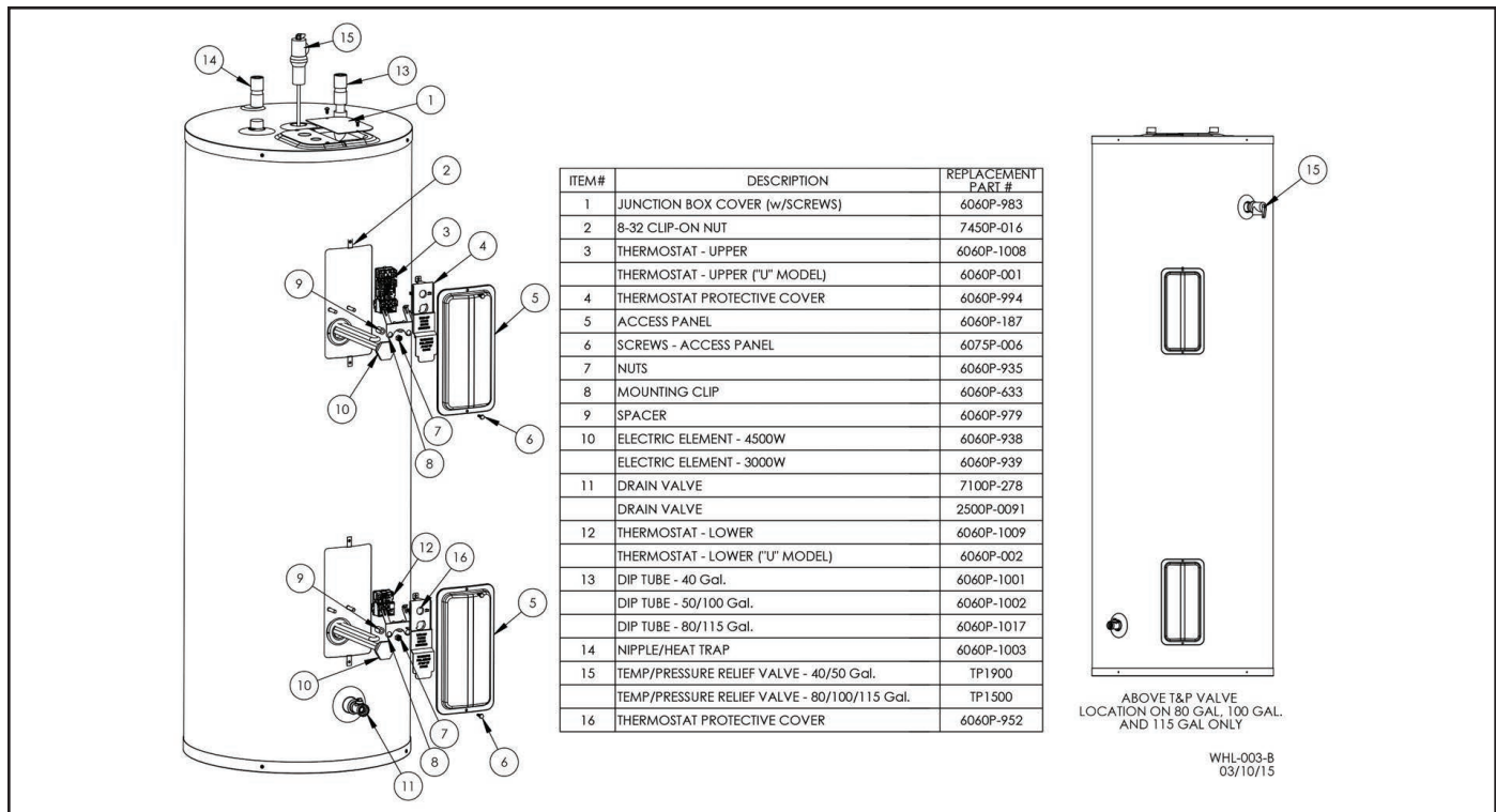
Figure 9 - Replacement Parts
