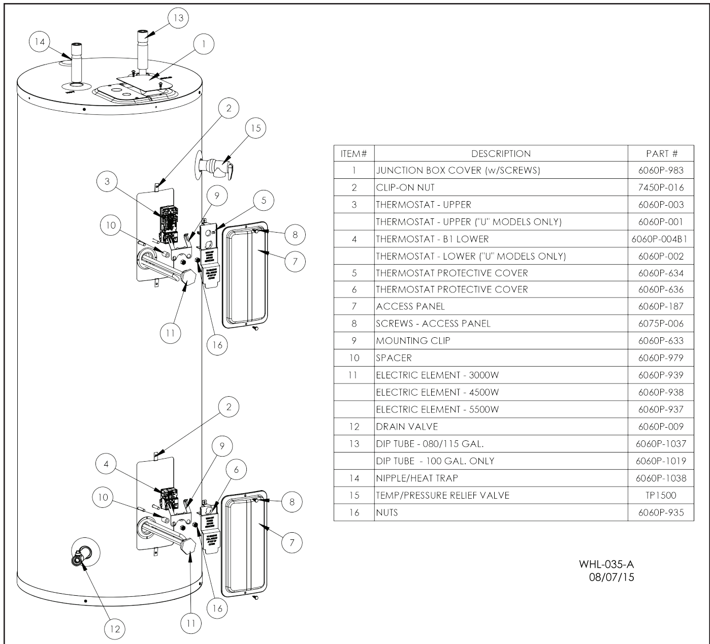
Figure 8 - Replacement Parts - Staged Operation
