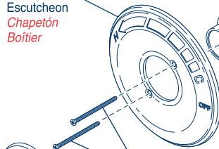
RP5417▲ Screws Tornillos Vis
