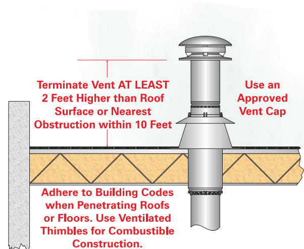
Figure 4.2: Vent Termination
