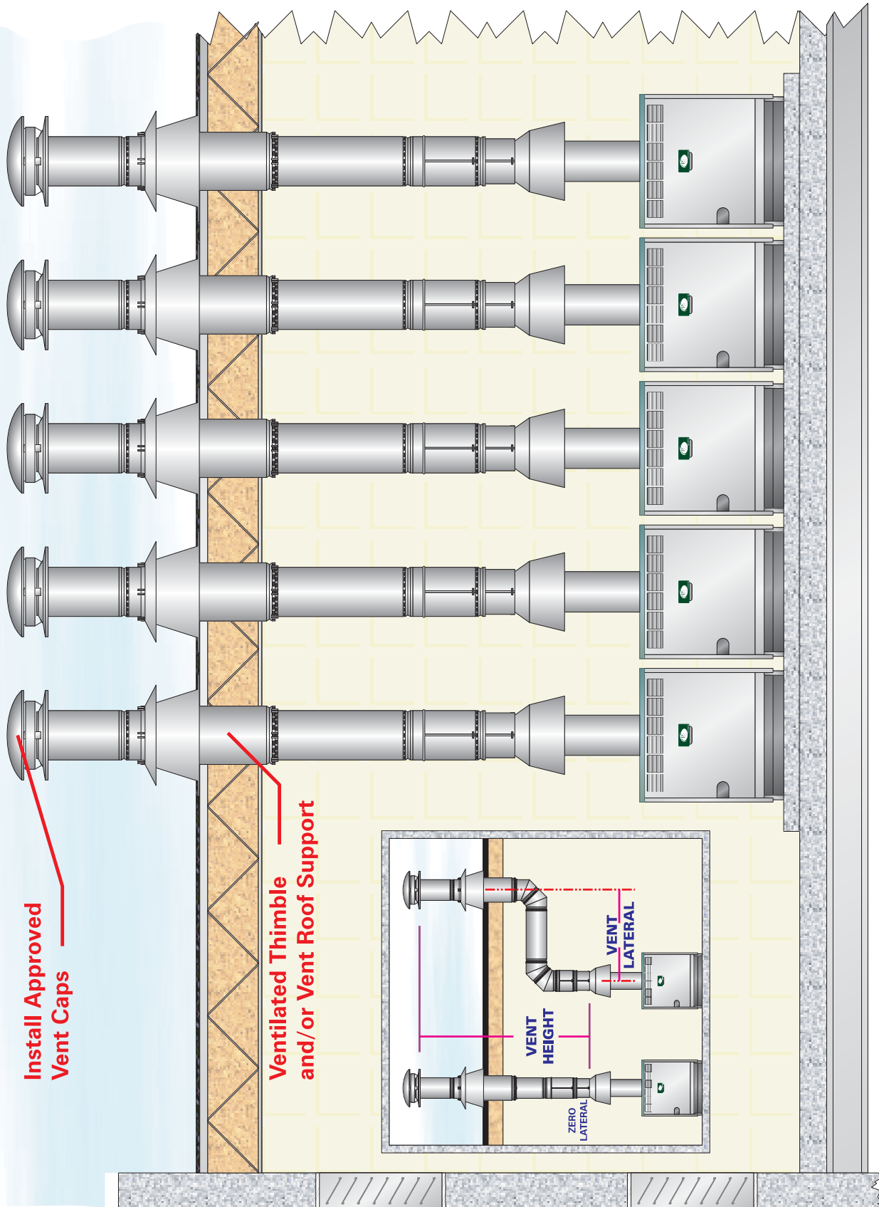
Figure 4.3: Individual Venting – See Table for Vent Sizing
