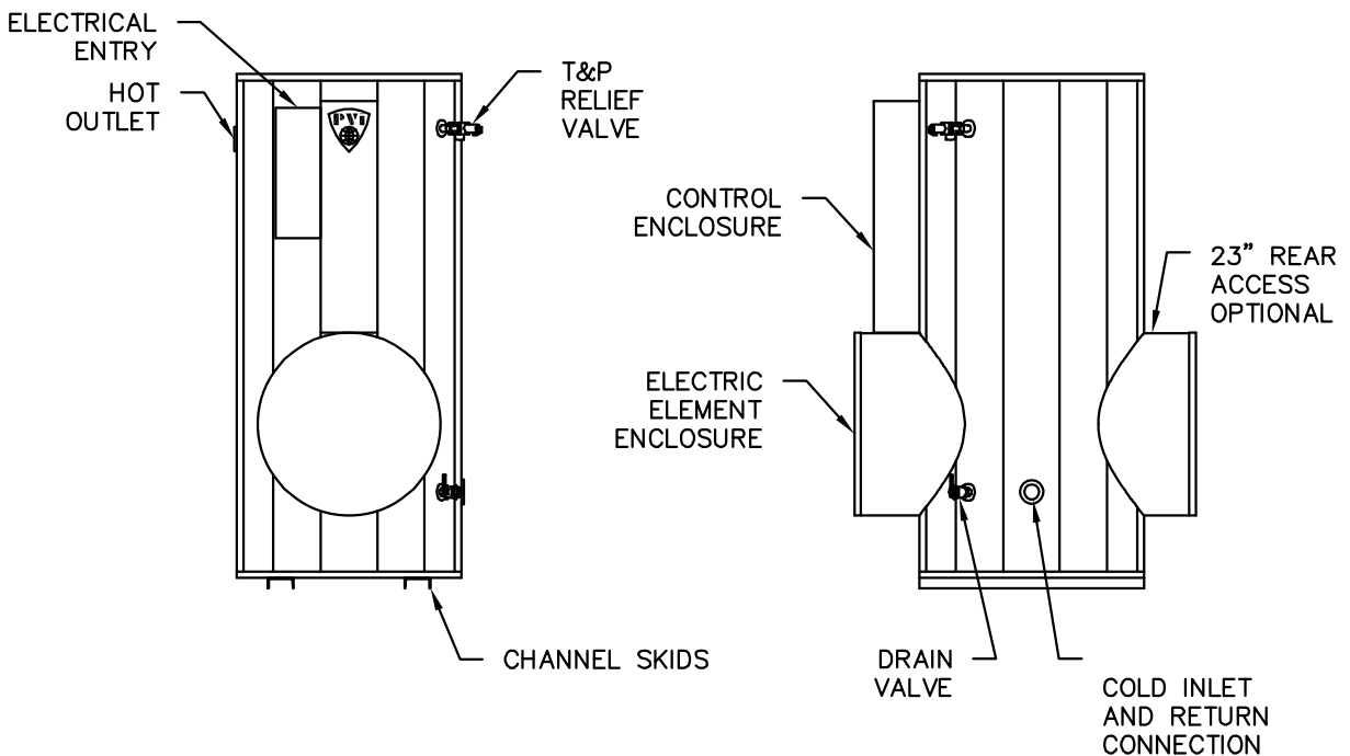
With 23" Diameter Tank Access FIGURE 2
