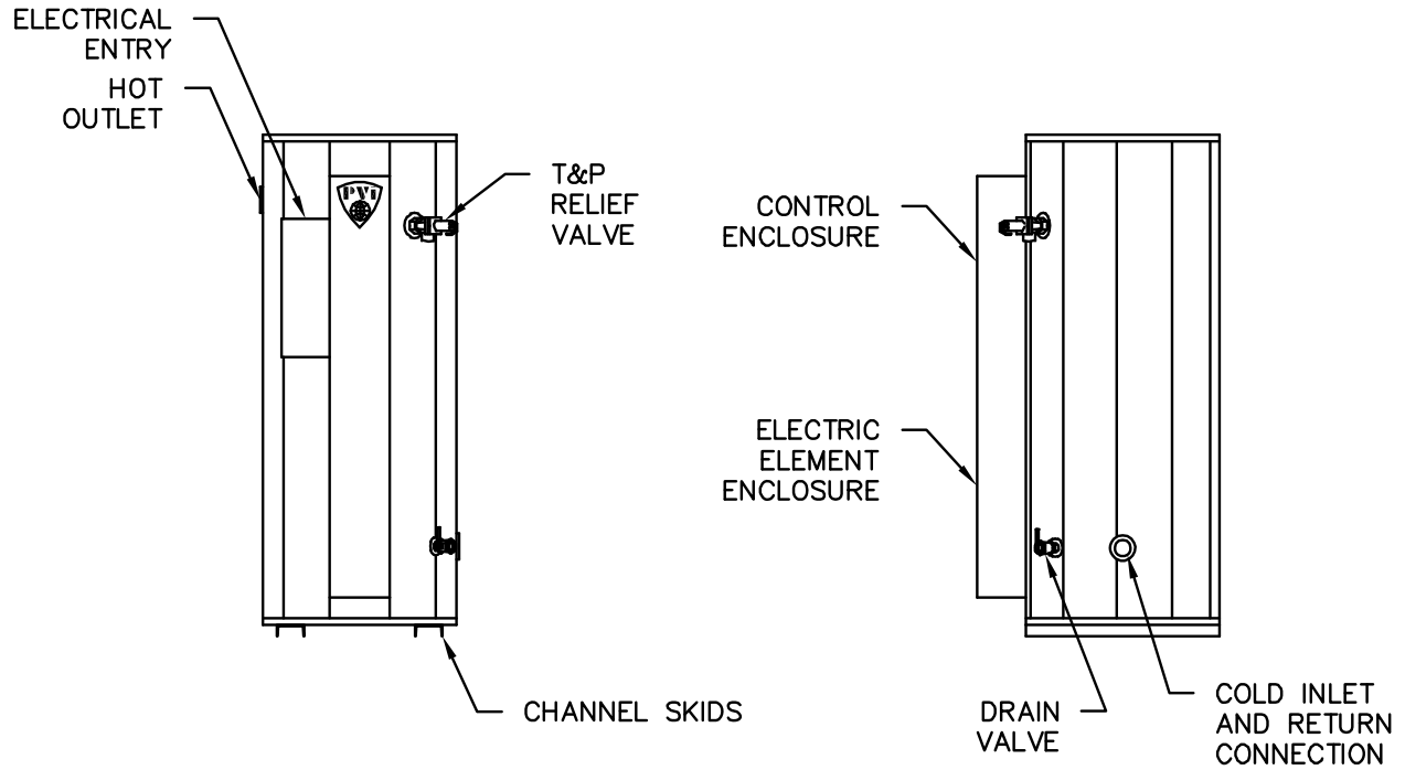
Without 23" Diameter Tank Access FIGURE 1
