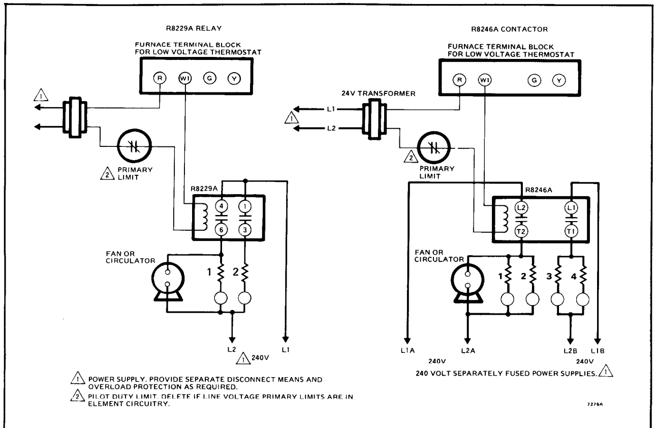
FIG. 9—COMBINATION RATED SINGLE-SPEED FAN CIRCUIT WITH PILOT DUTY LIMIT.
