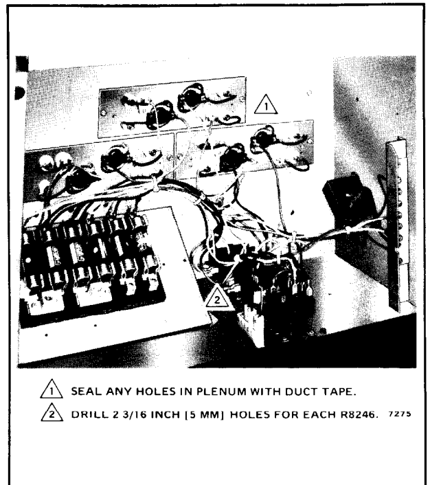
FIG. 5—INSTALL R8229A(S) AND R8246A(S).
