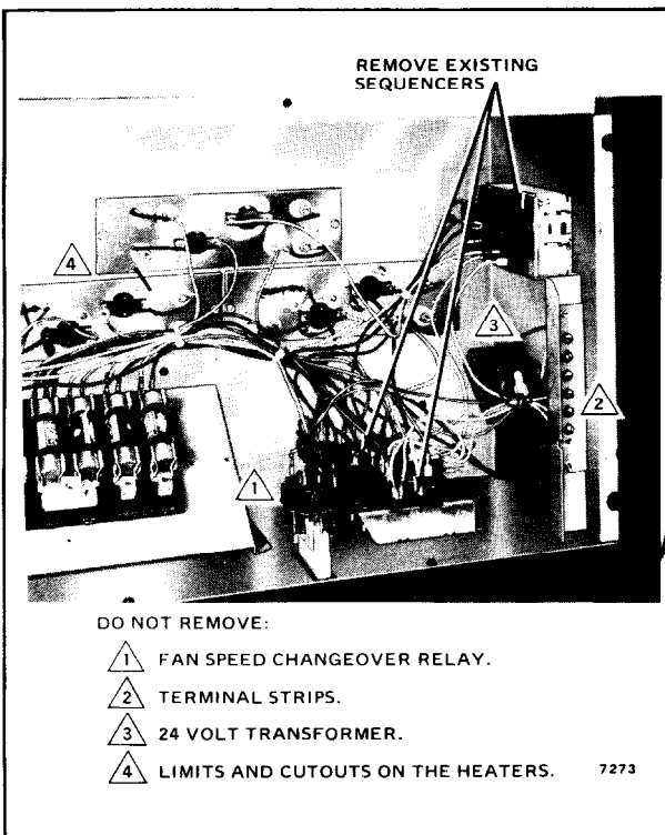
FIG. 3—REMOVE OLD SEQUENCERS.
