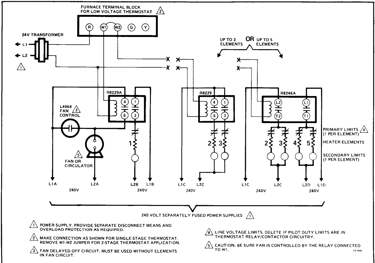
FIG. 7—DELAYED OFF FAN CONTROL IN ISOLATED FAN CIRCUIT WITH LINE VOLTAGE LIMITS.
