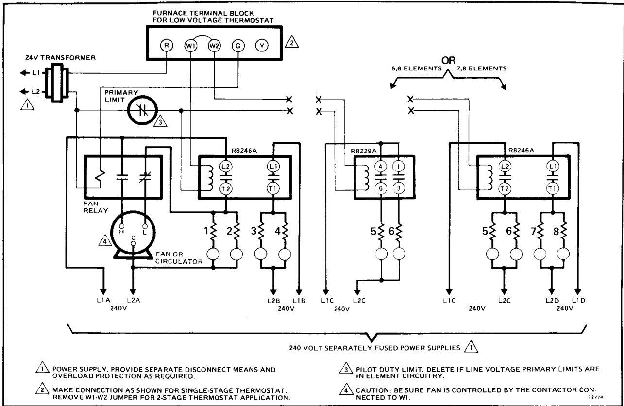
FIG. 6—COMBINATION RATED TWO-SPEED FAN CIRCUIT WITH PILOT DUTY LIMIT.
