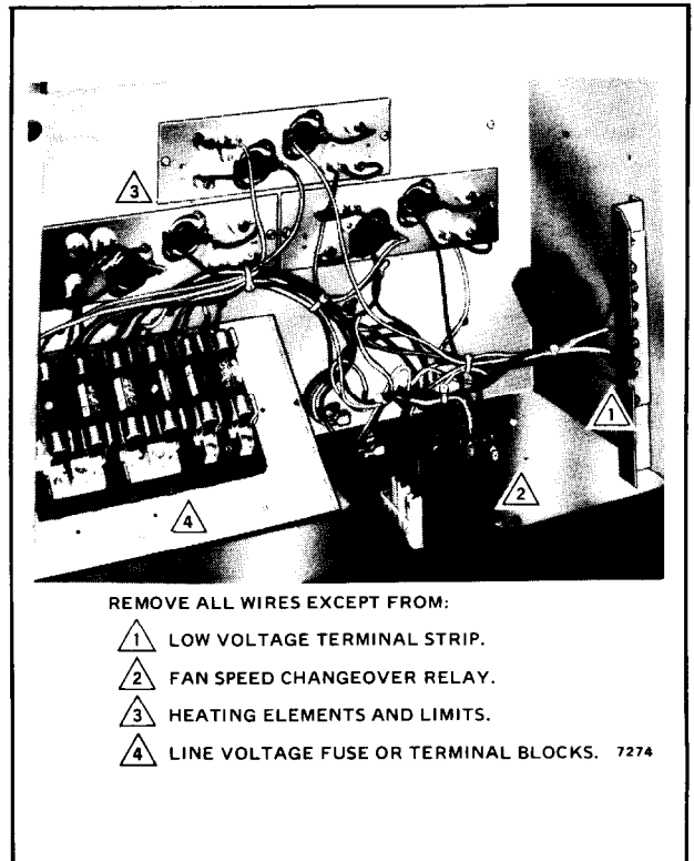
FIG. 4—REMOVE WIRING.
