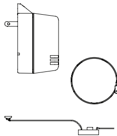
Plug-in transformer option (PT) includes Transformer (S53-338), Adapter (S53-339), and Grounding Kit (S53-349) for CAP-DCR Faucets
