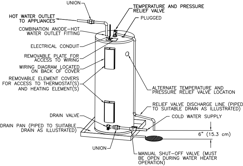
Figure 1B (Bottom Inlet Models)
