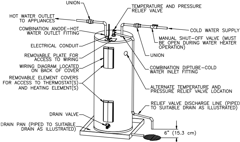
Figure 1A (Top Inlet Models)
